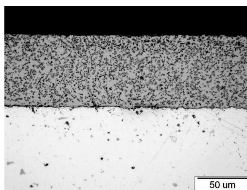
Fig. 10. Microstructure on the cross-section of coating produced at a current density of 6 A/dm 2
