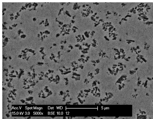
Fig. 7. Microstructure of coating produced at a current density of 8 A/dm 2
