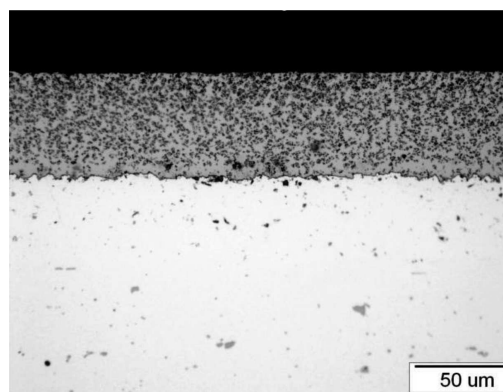
Fig. 9. Microstructure on the cross-section of coating produced at a current density of 4 A/dm 2
