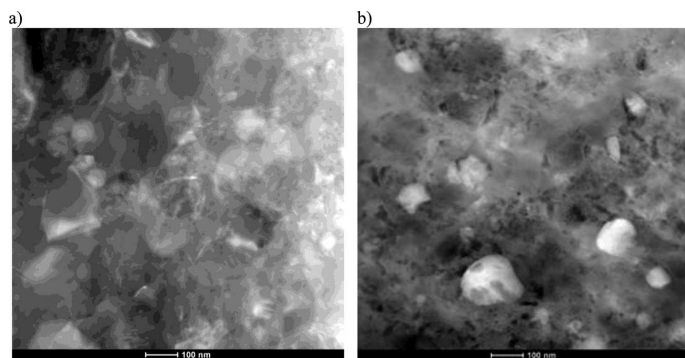
Fig. 3. Microstructure of the \text{AlMg}_1\text{SiCu} alloy (a) and composite material reinforced with 15 mass % halloysite nanotubes (b) produced by high-energy mechanical alloying, HAADF-STEM images
