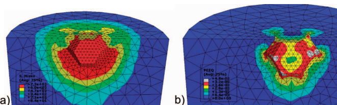
Fig. 9. Stress (a) and plastic strain (b) field around a loaded diamond crystal in Co-EF (200 N; HDP=75 \mu\text{m} )
