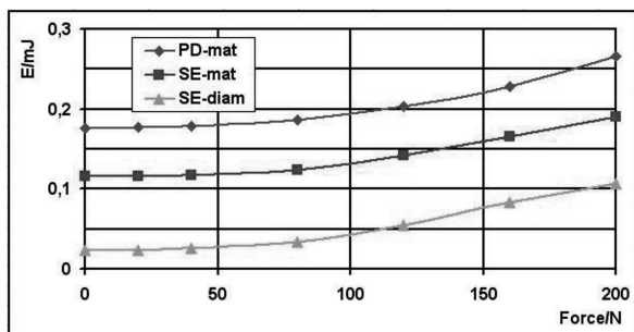
Fig. 11. Plastic strain (PD-mat) and elastic strain (SE-mat) energies of Co-EF, and elastic strain energy (SE-diam) of diamond (HDP=75 μm) as a function of normal load
