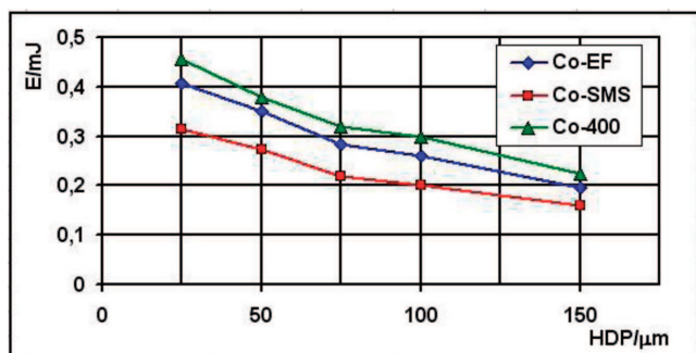
Fig. 6. Total strain energy as a function of height of diamond protrusion
