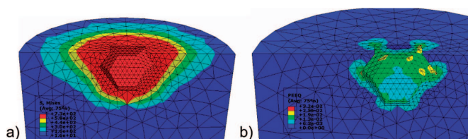
Fig. 8. Stress (a) and plastic strain (b) field around an unloaded diamond crystal in Co-EF (HDP=75 \mu\text{m} )
