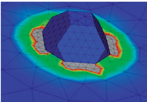
Fig. 3. Numerical model of a diamond particle with the strain zone
