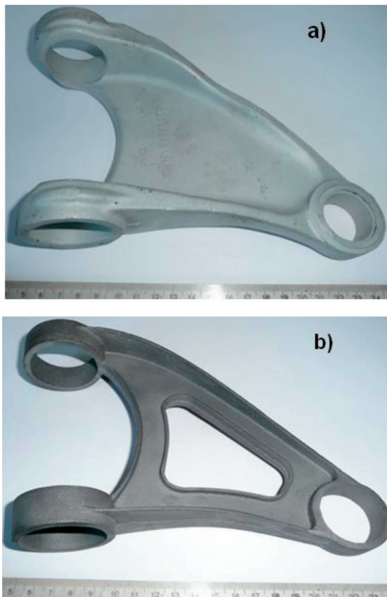
Fig. 6. Control arms: (a) forged aluminum alloy (weight 585 g) and (b) thin-walled ductile iron casting (weight 480 g)
