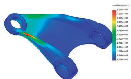
Fig. 13. Von Mises stress concentrations of control arm
