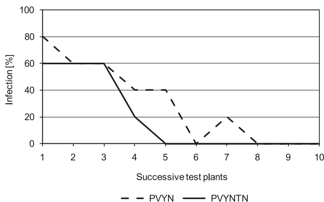
Fig. 4. The retention of PVY N and PVY NTN in M. persicae feeding following the virus acquisition
