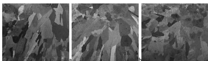
Fig. 2. CuSn10Zn2 bronze macrostructure. The initial alloy (a), after being modified by Kupmod B in the amount of 0.1% (b) and 0.2% of the metal stock mass (c)
