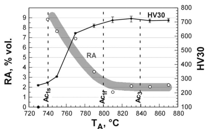
Fig. 4. Influence of annealing temperature on the volume fraction of retained austenite (RA) and hardness (HV30) of the 41MnSi6-5 steel
