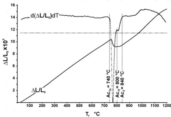
Fig. 2. Dilatometric curve of heating \Delta L/L_0 = f(T) with corresponding differential curve d(\Delta L/L_0)/dT = f(T) made for 41MnSi6-5 steel
