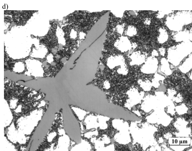
Fig. 5 (a-d). The microstructure of pressure die cast made of the tested silumin with the addition of V and Mo approximately: a – 0.1%, b – 0.2%, c – 0.3%, d – 0.4%: \alpha , \alpha + \text{Al}_9\text{Fe}_3\text{Si}_2 + \beta , \alpha + \text{Al}_2\text{Cu} + \text{AlSiCuFeMgMnNiVMo} + \beta
