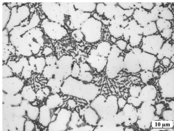
Fig. 4. The microstructure of 226 silumin obtained in the pressure die casting: \alpha, \alpha + \text{Al}_9\text{Fe}_3\text{Si}_2 + \beta, \alpha + \text{Al}_2\text{Cu} + \text{AlSiCuFeMgMnNi} + \beta
