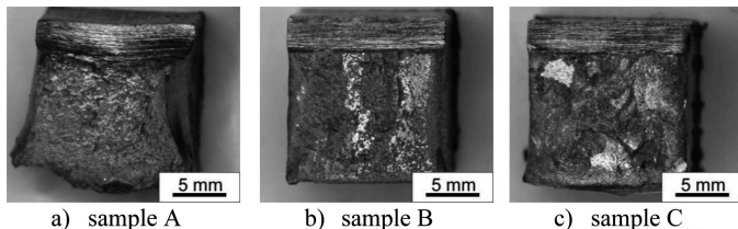
Fig. 3. Appearance of specimens of the cast steels after failure in -40°C
