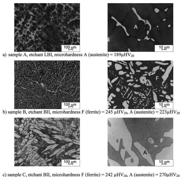
Fig. 1. Microstructure of the investigated stainless cast steels after the solution annealing heat treatment, LM
