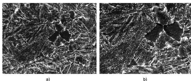
Fig. 5. SEM microstructure of the steel after quenching from 800°C and tempering at 650°C, sample etched in 4% \text{HNO}_3
