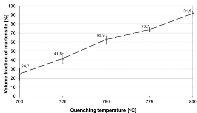
Fig. 6. The influence of quenching temperature on the martensite volume fraction in the steel
