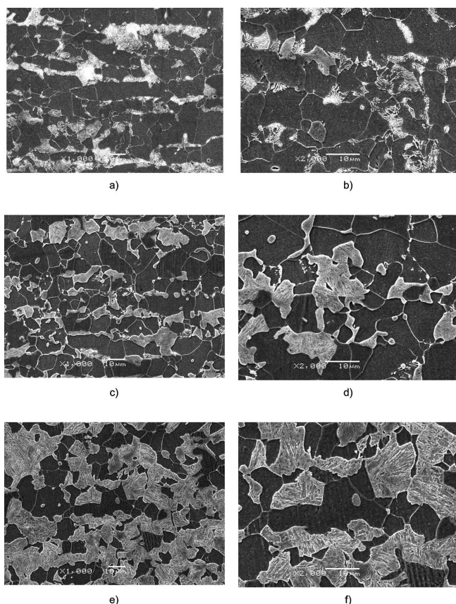
Fig. 2. SEM microstructure of the steel, etched in 4% \text{HNO}_3 : a, b) in delivery state; c, d) after quenching from 700°C e, f) after quenching from 750°C
