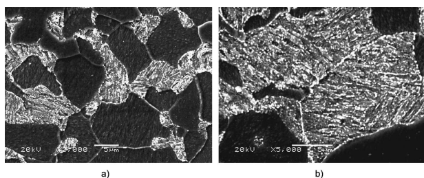
Fig. 4. SEM microstructure of the steel after quenching from 725°C and tempering at 650°C, sample etched in 4% \text{HNO}_3
