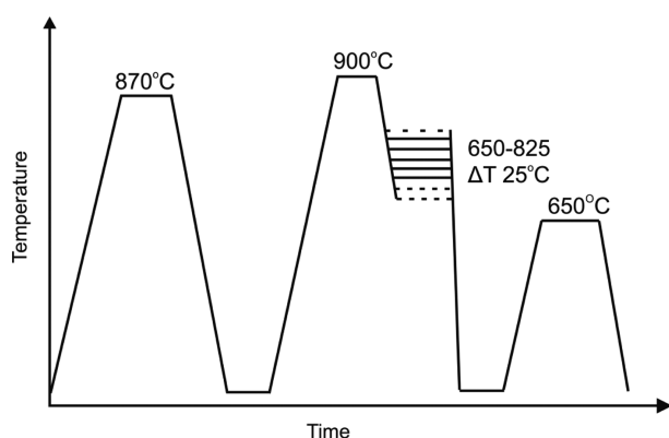
Fig. 1. Scheme of the heat treatment of the tested steel
