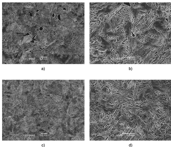
Fig. 3. SEM microstructure of steel etched in 4% \text{HNO}_3 : a, b) after quenching from 800°C; c, d) after quenching from 825°C
