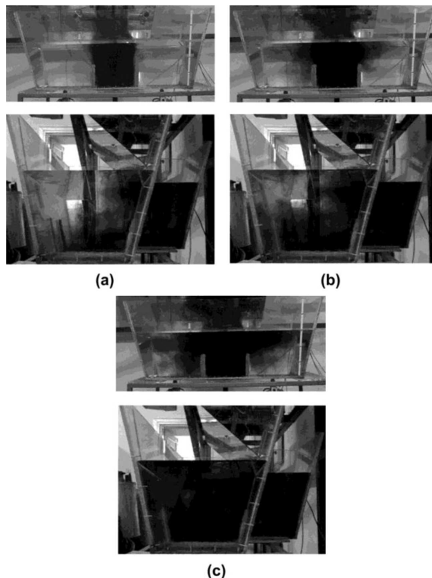
Fig. 6. Tracer propagation in tundish model (case C) after the time: (a) 10s, (b) 30s, (c) 60s
