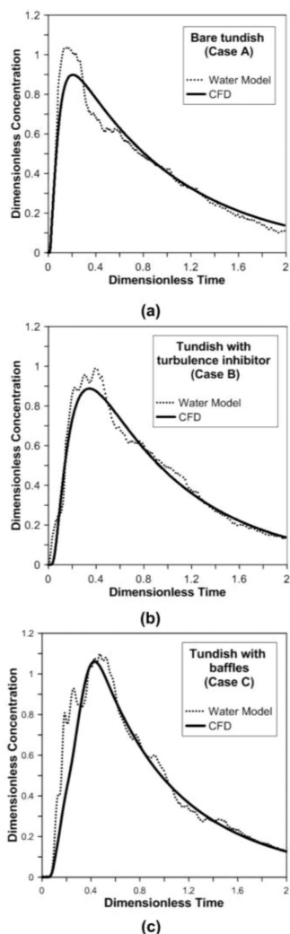
Fig. 3. Results coming from water model and CFD calculations (E-type curve): (a) case A, (b) case B, (c) case C
