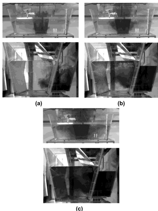
Fig. 4. Tracer propagation in tundish model (case A) after the time: (a) 10s, (b) 30s, (c) 60s
