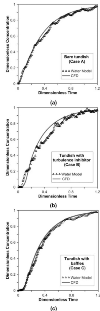
Fig. 2. Results coming from water model and CFD calculations (F-type curve): (a) case A [14], (b) case B [19], (c) case C
