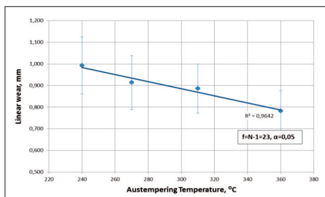
Fig. 6. The wear of test samples as a function of the austempering temperature
