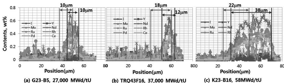
Fig. 4. EMPA line scanning for fission products in used cladding hull tubes with various burn-ups; (a) 27,000 MWd/tU, (b) 37,000 MWd/tU, and 58,000 MWd/tU
