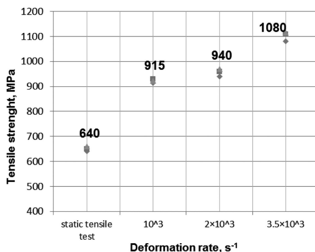
Fig. 2. The effect of the deformation rate on the ultimate tensile strength of the investigated steel
