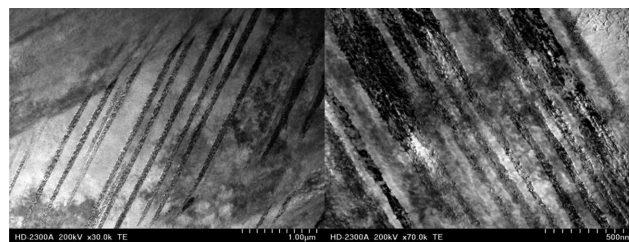
Fig. 6. STEM image on area containing mechanical twins in a sample after dynamic deformation with a rate of 30 m/s
