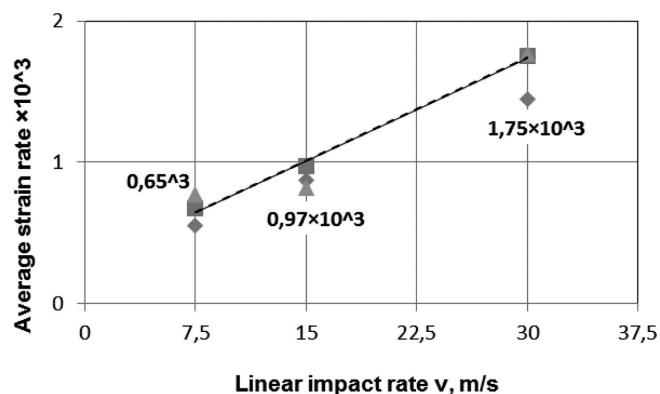
Fig. 1. Dependence between the impact linear velocity and the average deformation rate
