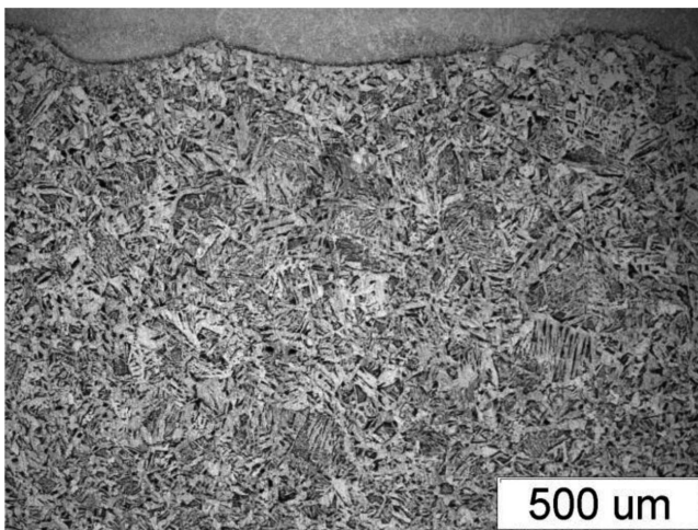
Fig. 2. High amount of acicular ferrite in weld (73%) after Ar micro-jet cooling
