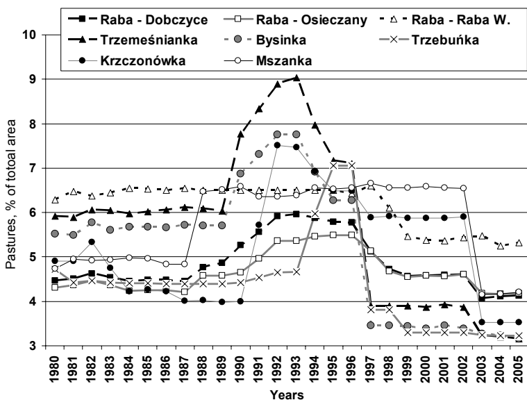
Fig. 3. Changes in the surface area of pastures in the upper Raba River basin
