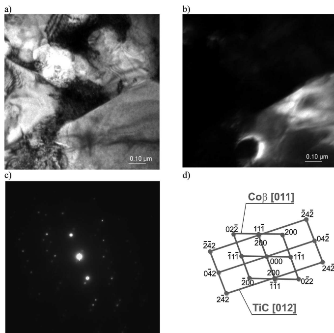
Fig. 6. Structure of cermet substrate: a) bright field; b) dark field from (\bar{2}00) TiC and (11\bar{1}) Co reflex; c) diffraction pattern from area b and d) solution of the diffraction pattern
