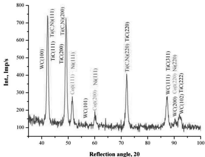
Fig. 5. X-ray phase analysis of the cermet substrate (Bragg-Brentano geometry)
