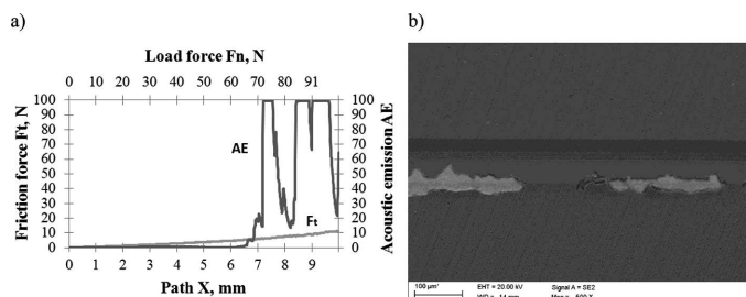
Fig. 9. Scratch test results of the gradient (Ti,Al)N coating surface a) diagram of the dependence of the acoustic emission (AE) and friction force Ft, b) characteristic failure around L_c zone(SEM)
