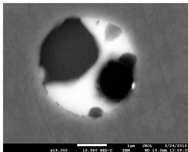
Fig. 3. The spherical shape of nonmetallic inclusions in the modified G17CrMo5-5 cast steel
