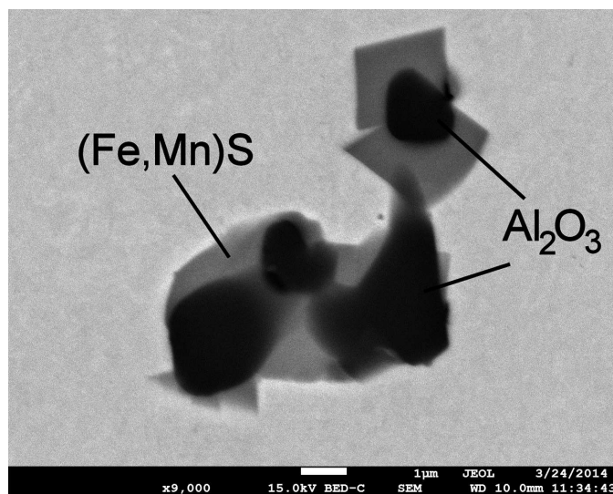
Fig. 2. The shape of nonmetallic inclusions in the unmodified G17CrMo5-5 cast steel
