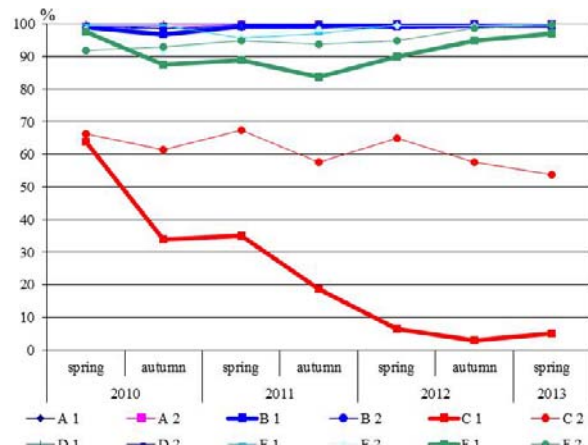
Fig. 3. Changes of the turf cover in the study years; 1 – grazed by sheep; 2 – non-grazed (abandoned grassland); A – community with species ChAll. Vicio lathyroidis-Potentillion argenteae involving species ChCl. Molinio-Arrhenatheretea ; B – community dominated by species ChCl. Koelerio glaucae-Coryneporetea canescentis involving species ChCl. Molinio-Arrhenatheretea ; C – Ass. Spergulo-Coryneporetea ; D – community with the domination of Calamagrostis epigejos (Ass. Coryneporetea-Silenetum tataricae ); E – community with Poa pratensis involving species ChCl. Molinio-Arrhenatheretea ; F – community with species ChAll. Vicio lathyroidis-Potentillion argenteae dominated by species ChCl. Koelerio glaucae-Coryneporetea canescentis ; source: own study
