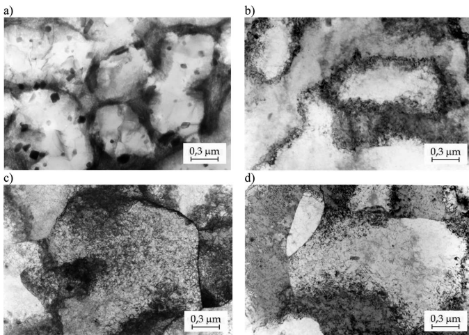
Fig. 6. The microstructure of 6063 alloy after plastic deformation in the temperature of: a,b) T_{\varepsilon} - 200^{\circ}\text{C} , \dot{\varepsilon} = 0,001 \text{ s}^{-1} ; c,d) T_{\varepsilon} - 300^{\circ}\text{C} , \dot{\varepsilon} = 0,001 \text{ s}^{-1}
