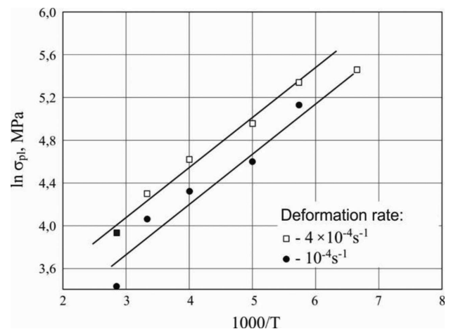
Fig. 8. The influence of temperature and deformation rate on the value of flow strain of 6005 aluminium alloy – linear extrapolation of experimental results in temperature range of 150-350^{\circ}\text{C}
