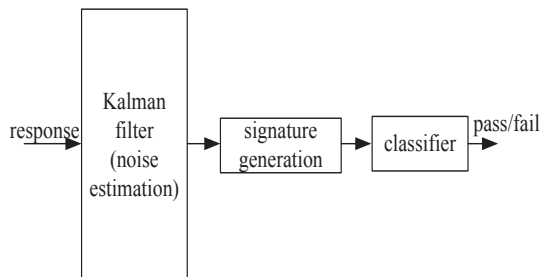
Fig. 1. Signature analysis scheme using Kalman filtering.
