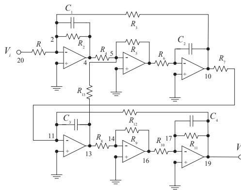
Fig. 5. Leapfrog filter.
