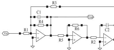
Fig. 9. Tow-Thomas filter.
