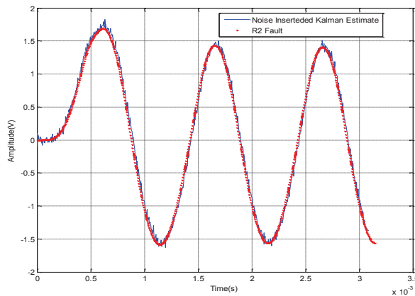
Fig. 7. Leapfrog Filter: The Kalman filter based method for realization of the R2 parametric fault response (red dotted line) by using the fault-free response plus Gaussian white noise with a proper variance (blue solid line). X-axis denotes the time (s), Y-axis denotes the amplitude (v).
