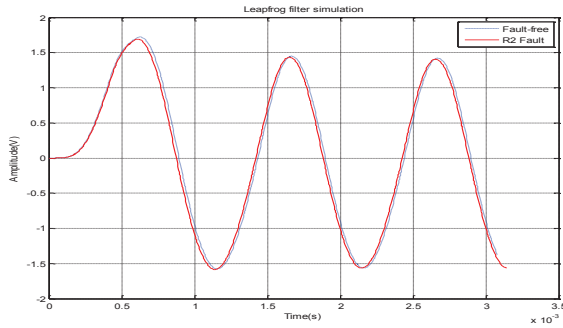
Fig. 6. Leapfrog filter: Fault-free response (blue dotted line) and R2 parameter fault response (red solid line). X-axis denotes the time (s), Y-axis denotes the amplitude (v).
