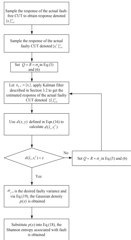
Fig. 4. Algorithm for fault signature extraction.
