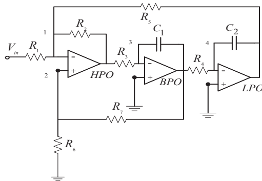
Fig. 8. State variable filter.
