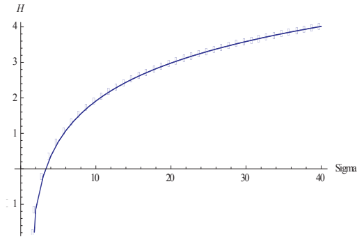
Fig. 2. Signature extraction using Shannon's entropy. X-axis denotes the variance of Gaussian distribution, Y-axis denotes Shannon's entropy
