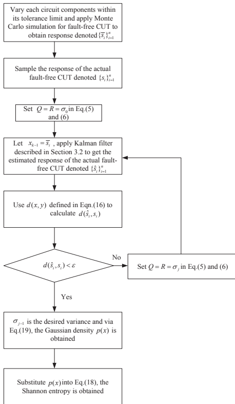
Fig. 3. Algorithm for fault-free signature extraction.
