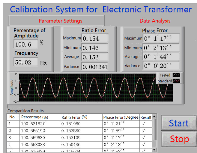
Fig. 7. Data analysis interface of the calibration system.
