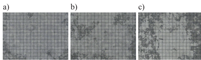
Fig. 8. Surface of Al-Si coating after the heat treatment at 450°C during a) 30 min, b) 180 min, c) 1440 min and influence of snow mud during 8 months
