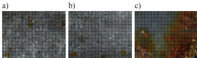
Fig. 12. Surface of Al-Si coating after the heat treatment at 500°C during a) 30 min, b) 180 min, c) 1440 min and influence of snow mud during 12 months
