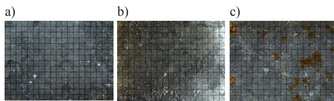
Fig. 9. Surface of Al-Si coating after the heat treatment at 450°C during a) 30 min, b) 180 min, c) 1440 min and influence of snow mud during 12 months
