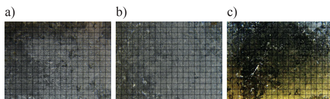
Fig. 6. Surface of Al-Si coating after the heat treatment at 250°C during a) 30 min, b) 180 min, c) 1440 min and influence of snow mud during 12 months
