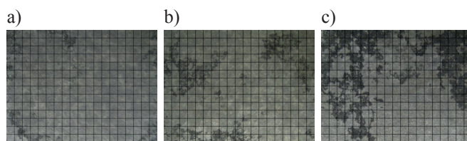
Fig. 7. Surface of Al-Si coating after the heat treatment at 450°C during a) 30 min, b) 180 min, c) 1440 min and influence of snow mud during 4 months
