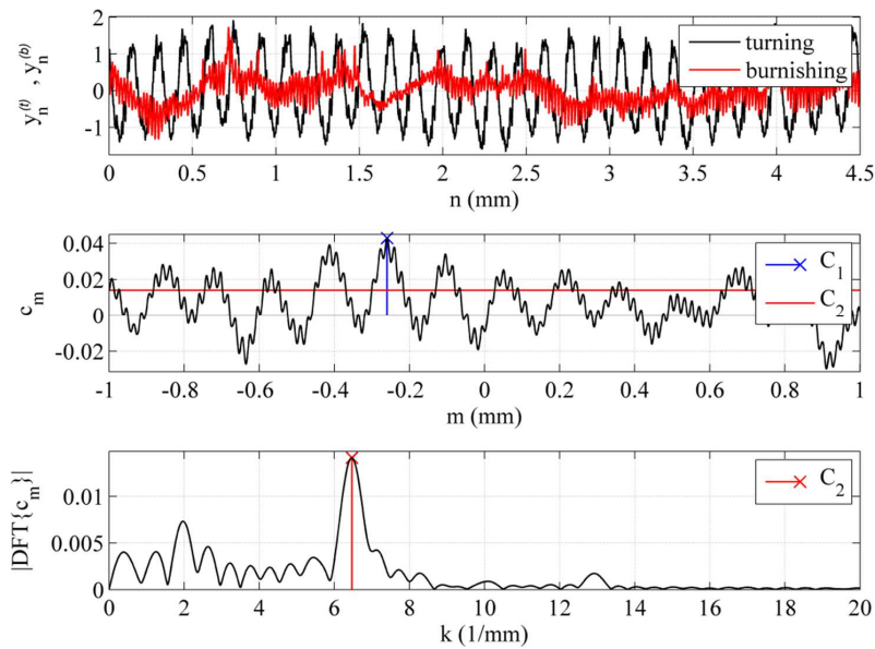
Fig. 6. The results for turned and burnished ( F = 200\text{ N} , f = 0.02\text{ mm/rev.} ) Sverker 21 tool steel: the measured signals (top), the cross-correlation function with marked value of C_1 = 0.043 (middle) and the DFT amplitude spectrum with denoted value of C_2 = 0.014 (bottom).
