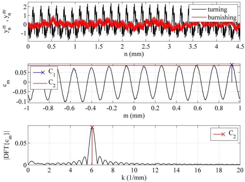
Fig. 4. The results for turned and burnished ( F = 180 N, f = 0.02 mm/rev.) Vanadis 6 tool steel: the measured signals (top), the cross-correlation function with marked value of C_1 = 0.089 (middle) and the DFT amplitude spectrum with denoted value of C_2 = 0.085 (bottom).
