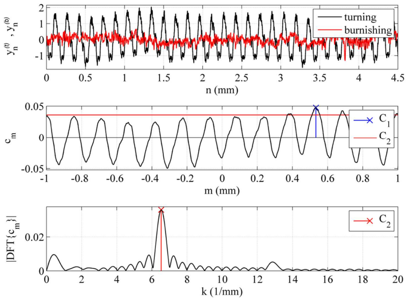
Fig. 5. The results for turned and burnished ( F = 180 N, f = 0.02 mm/rev.) Sverker 21 tool steel: the measured signals (top), the cross-correlation function with marked value of C_1 = 0.048 (middle) and the DFT amplitude spectrum with denoted value of C_2 = 0.036 (bottom).
