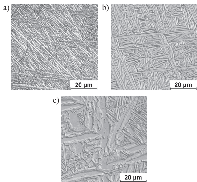
Fig. 7. Microstructure of Ti-6Al-4V alloy (DIC) after water quenching from the temperature of \beta range (a) and following annealing at 900°C for 0,5 h (b) and 1 h (c)
