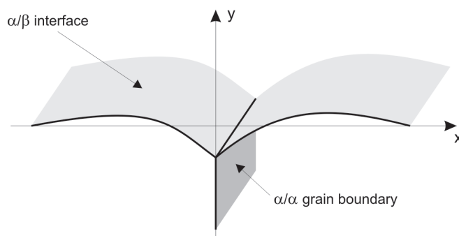
Fig. 9. Scheme of \beta phase grain growth by „grooving” of \alpha/\beta interphase [6,20,21]
