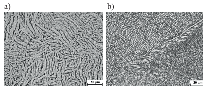
Fig. 6. Microstructure of Ti-6Al-4V (a) and Ti-6Al-2Mo-2Cr (b) alloys after \beta quenching and plastic deformation in the \alpha + \beta \rightarrow \beta range (longitudinal cross-section)
