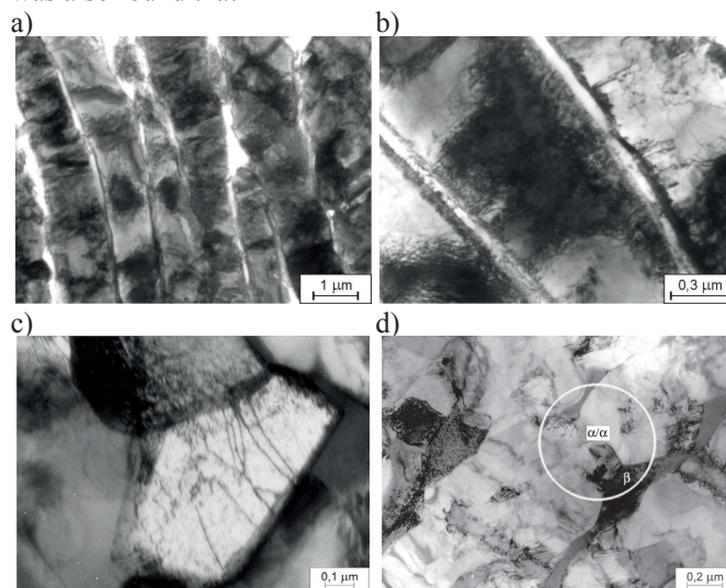
Fig. 8. Microstructure (TEM) of Ti-6Al-4V alloy after TMP - elongated \alpha_D grains with high dislocation density (a, b), fragmentation of \alpha_D grains by high-angle boundary formation (c) and „grooving” of \alpha/\beta interface (d)
