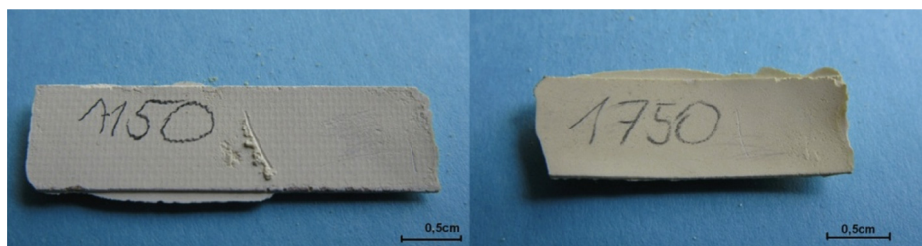
Fig. 20. The photograph of samples preheated at 1150 and 1750°C after the “scratch test”
