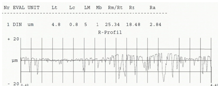
Fig. 32. An example of the measured roughness profile of the mould surface
