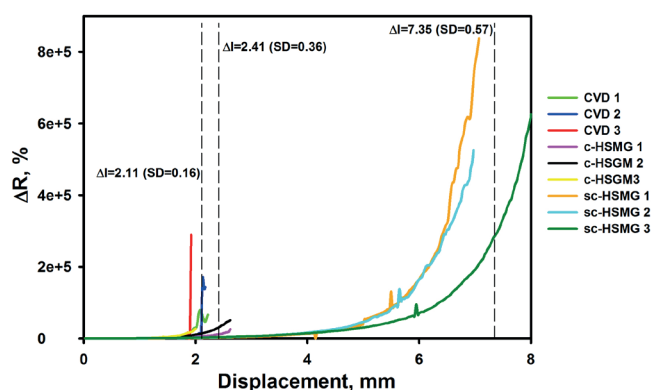
Fig. 7. Evolution of the electrical resistance during tensile testing of the examined graphene samples
