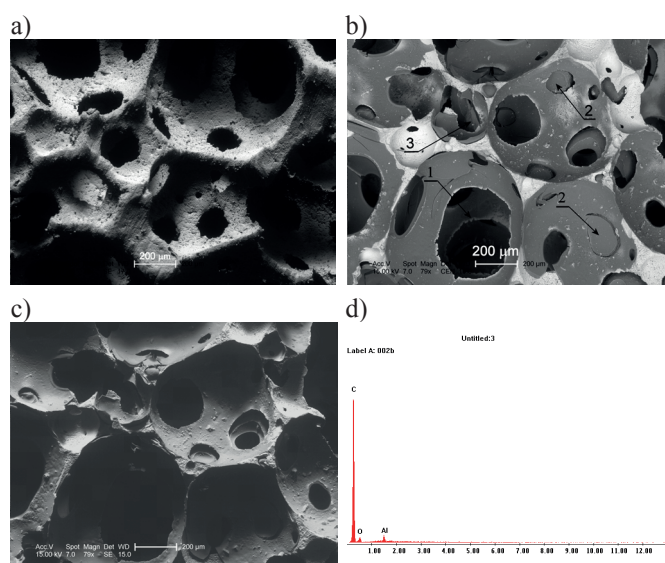
Fig. 2. Ceramic foam surface before (a) and after (b, c) carbon precursor introduction and its pyrolysis; element distribution (d), SEM: 1 – open pores for matrix infiltration, 2 – pores closed with glassy carbon, 3 – glassy carbon piece inside ceramic spheroid
