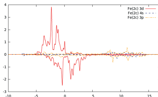
Figure 6. PDOS curves for Fe(2c)
