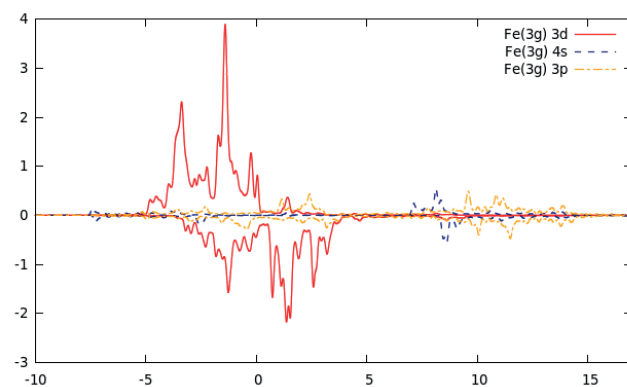
Figure 7. PDOS curves for Fe(3g)
