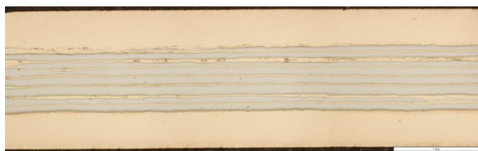
Fig. 11. Microstructure of Cu-Fe wire of diameter a) 4.1 mm, b) 1.78 mm, longitudinal section
