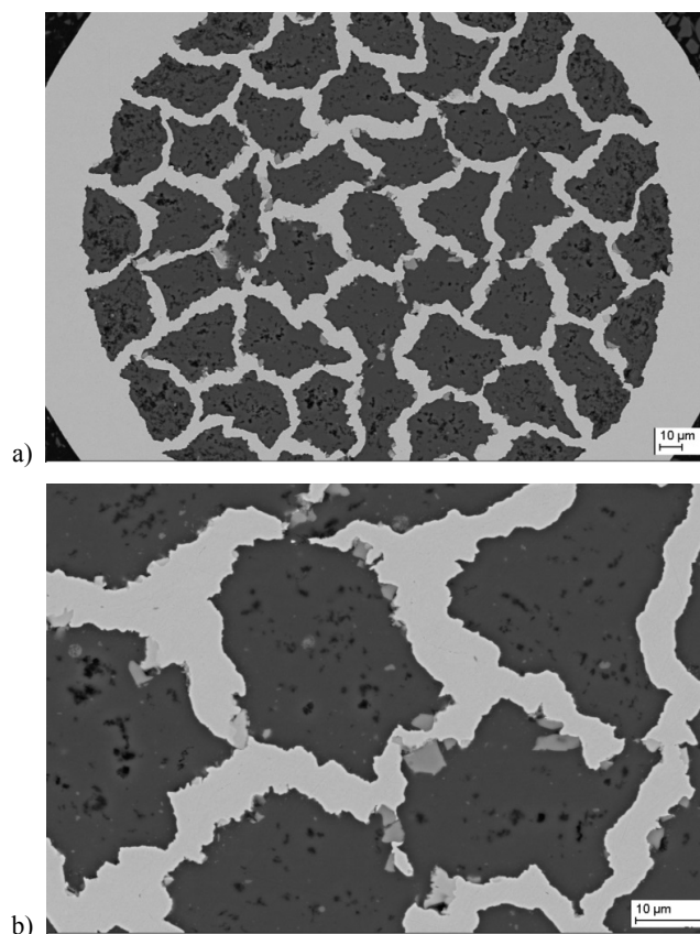
Fig. 4. Microstructure of CuAl wire of diameter 0.34, polished cross-section, SEM, a) magnif. 1000×, b) magnif. 3000×
