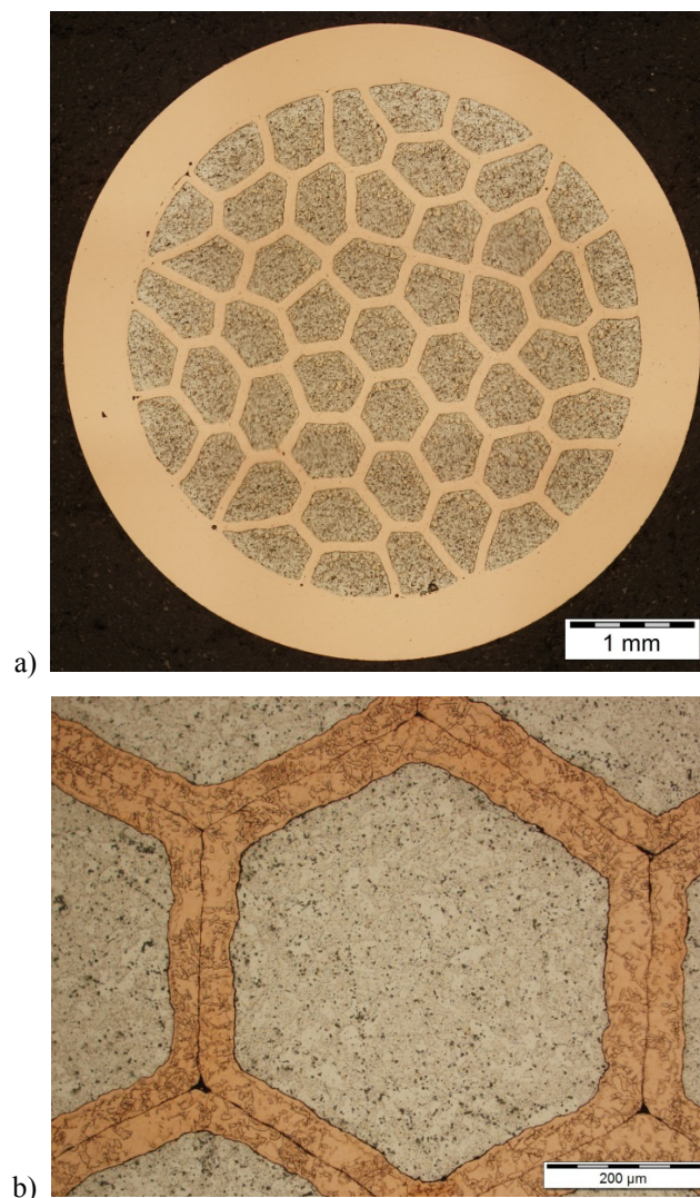
Fig. 1. Microstructure of Cu-Al wire of diameter 5.1 mm, a) magnif. 60 \times , b) magnif. 200 \times
