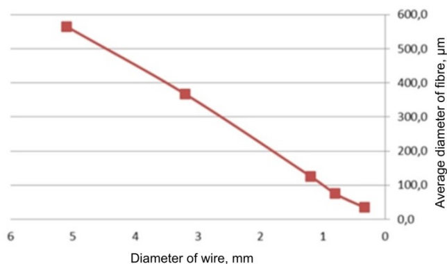
Fig. 2. Changes of average diameter of Al fibres vs outer diameter of composite wire during drawing
