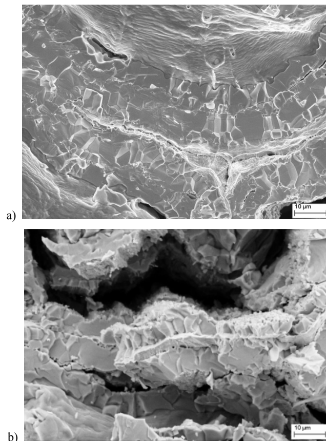
Fig. 5. Fracture of CuAl wire of diameter 1.4 additionally annealed in temperature 500°C/1h, SEM, a) magnif. 3000×, b) magnif. 3000×
