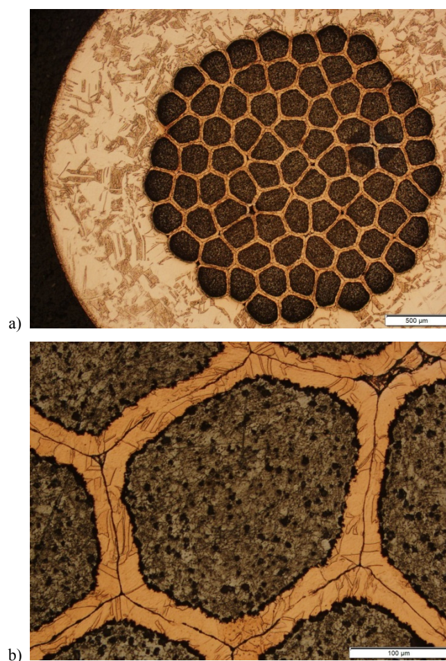
Fig. 8. Microstructure of Cu-Fe wire of diameter 4.1mm, cross-section, a) magnif. 50\times , b) magnif. 400\times
