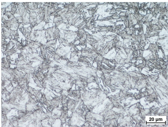
Fig. 2. The microstructure of S690QL steel after heat treatment, light microscopy
