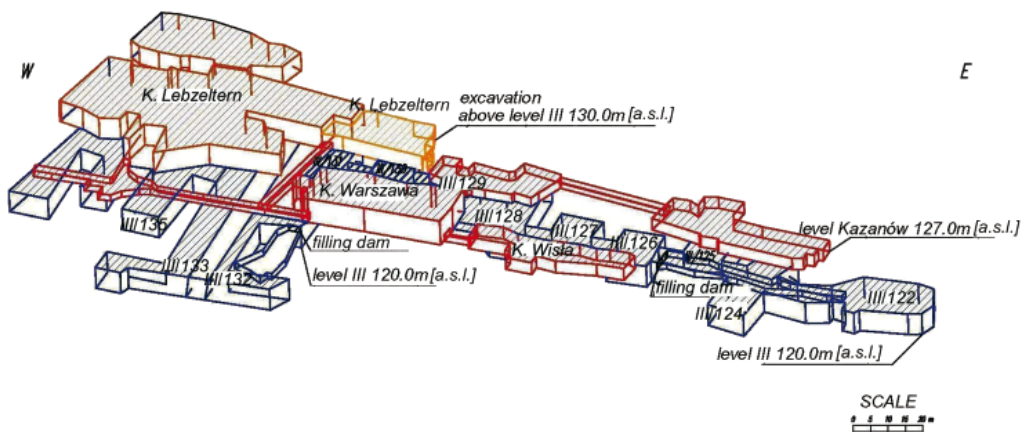
Fig. 1. Diagram of the spatial outlay of the Warszawa, Wisła, Budryk, Lebzeltern, and Upper Witos Chambers at the Kazanów mid-level and the Witos Chambers at Level III
