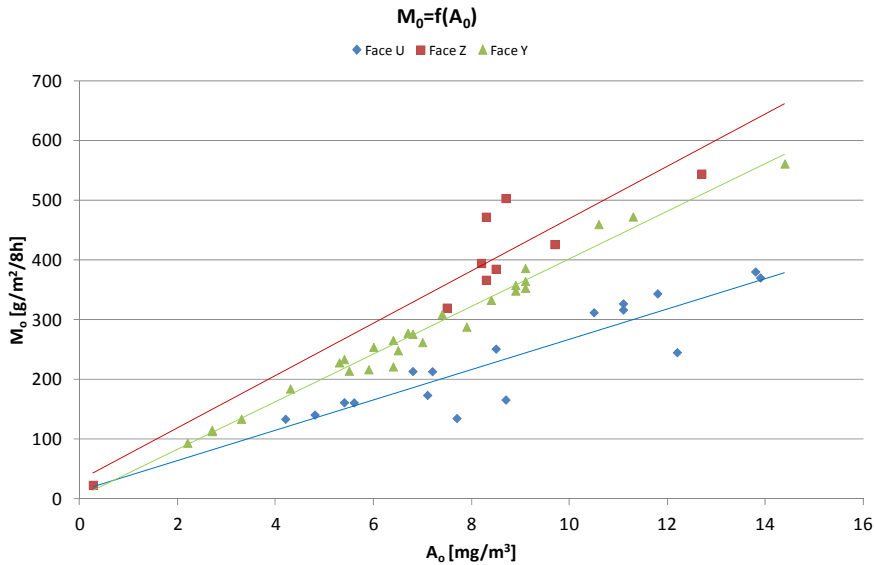
Fig. 10. Dependency of the coal dust depositing intensity ( M_o ) on the average dust source intensity ( A_o )
