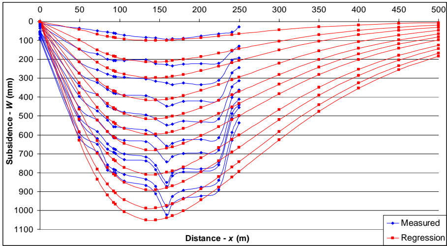
Fig. 29. Subsidence curves of the measured and approximated values, for the case of coal seam no. 3, face no. 138 and 139, Petřila Mine
