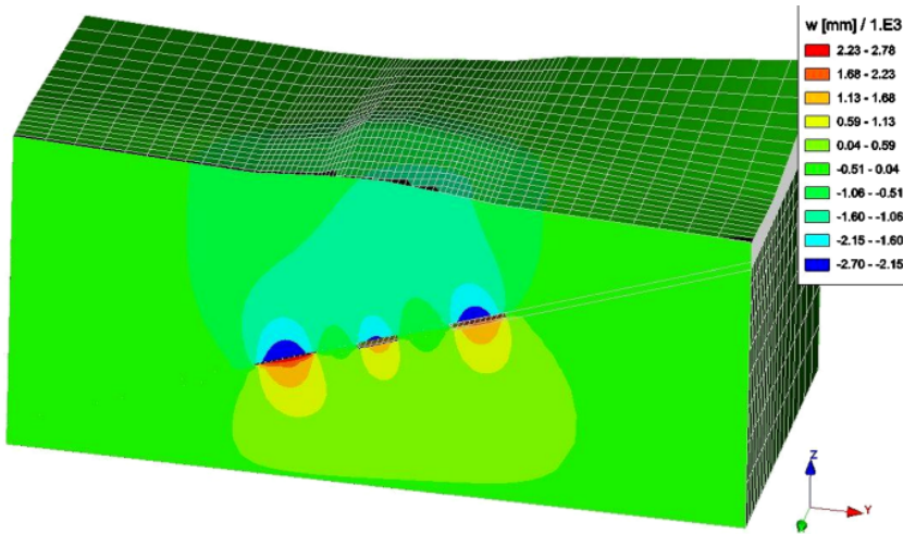
Fig. 15. Scalar representation of the subsidence, following the principal profile (in the centre of the “mining voids”) w, in mm
