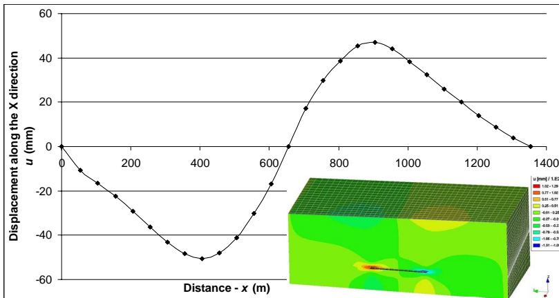
Fig. 24a. Horizontal displacements after X axis, obtained from 3D numerical modelling
