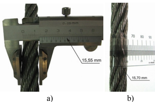
Fig. 3. Methods of measuring rope diameter: a) – a vernier calliper, b) – a ruler with an appropriate scale which takes into account the number \pi
