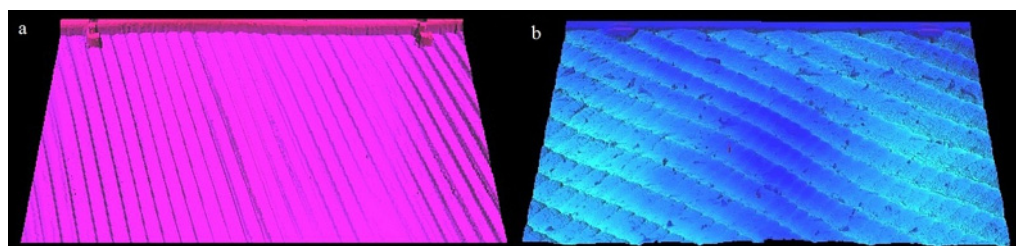
Fig. 9. 3D images of rope surface projections: a) – locked-wire rope with 23 “Z” wires in the outer layer, b) – 8-strand fiber rope
