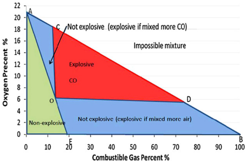
Fig. 3. CO explosive triangle
