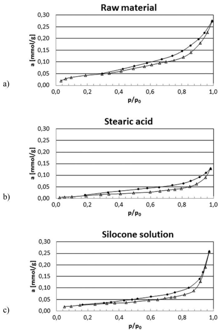
Fig. 1. Water vapour adsorption isotherm for limestone powder a) raw, b) hydrophobized in stearic acid vapour, c) hydrophobized in silocone solution ( \Delta – sorption; \bullet – desorption curve)
