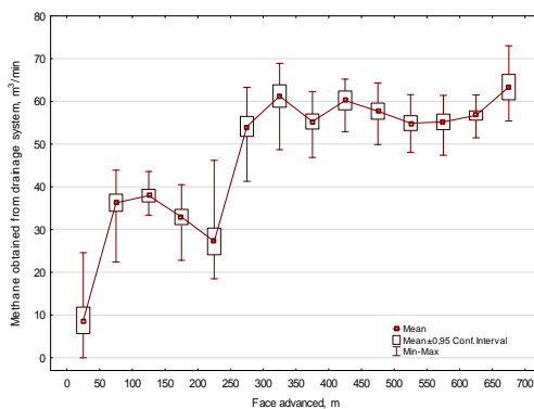
Fig. 25. Changes in the amount of captured methane compared with the face advance of longwall B-11
