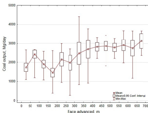
Fig. 27. Changes in coal output compared with the face advance of longwall B-11
