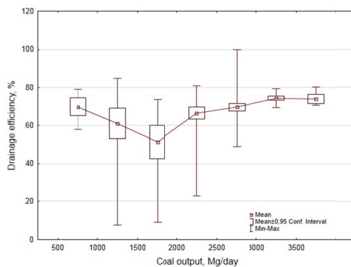
Fig. 29. Changes in the efficiency of methane drainage compared with coal output from longwall B-11
