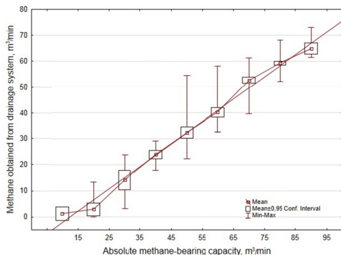
Fig. 30. Changes in the amount of captured methane compared with absolute methane-bearing capacity in longwall B-11
