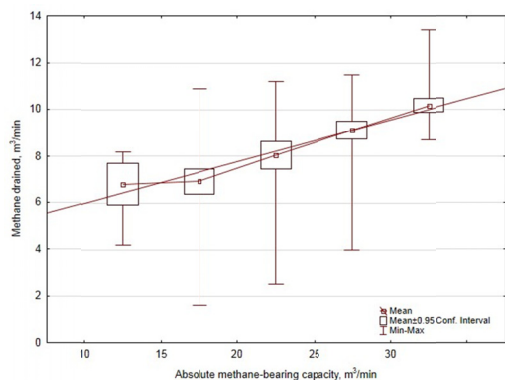
Fig. 12. Changes in the amount of drained methane compared with absolute methane-bearing capacity in longwall D-2
