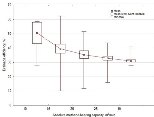
Fig. 13. Changes in the efficiency of methane drainage compared with absolute methane-bearing capacity in longwall D-2
