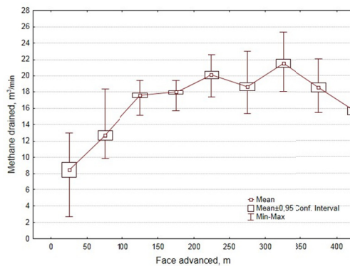
Fig. 17. Changes in the amount of drained methane compared with the face advance of longwall 2 in seam 506
