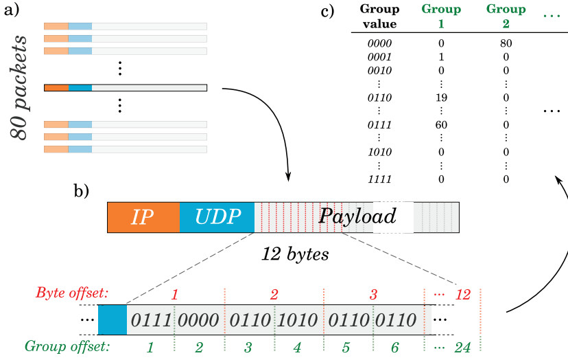
Fig. 1: Feature extraction in the KISS algorithm: for each packet in an 80-packet window (a), the first 12 bytes of UDP payload are divided into 24 groups of 4 bits each (b). Number of occurrences of distinct values in given group is counted for the whole packet window (c).
