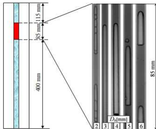
Figure 3: Registration area (marked rectangle) and exemplary observed flow structures ( w_{sg} = 0.14-0.16 m/s and w_{sl} = 0.70-0.75 m/s.)
