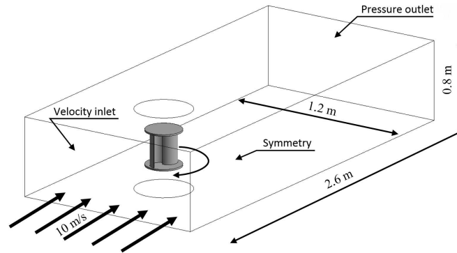
Figure 2: Computational domain.
